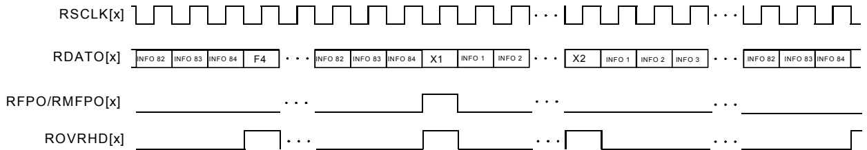
Figure 46 Framer Mode with DS3 Receive Output Stream
