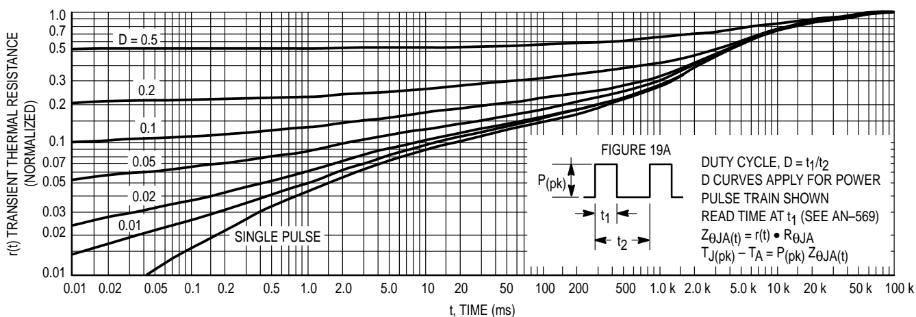
Figure 16. Thermal Response
