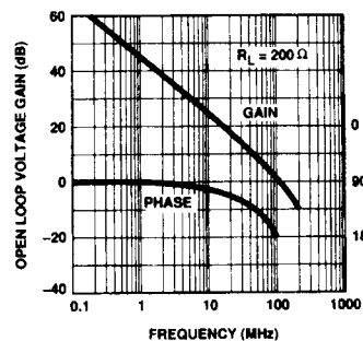
Open Loop Voltage Gain vs Frequency
