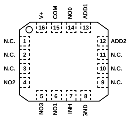
ISL43640 (QFN) TOP VIEW
