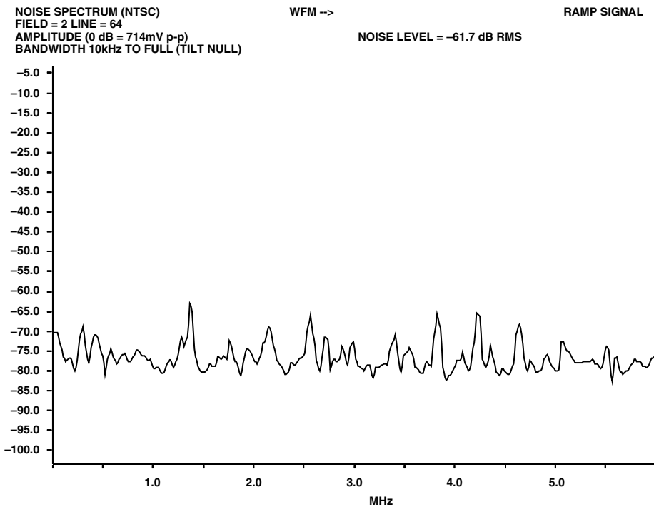
Figure 96. NTSC SNR Ramp Measurement
