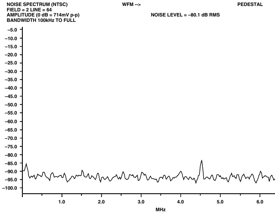
Figure 95. NTSC SNR Pedestal Measurement
