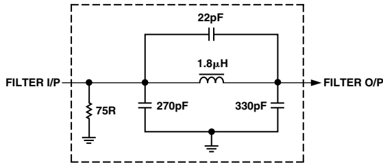
Figure 79. Output Filter
