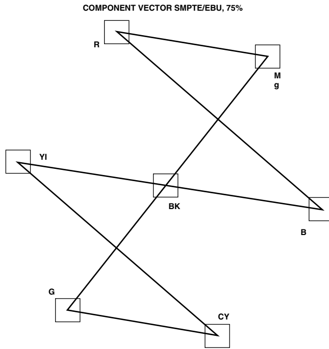
Figure 101. PAL YUV Vector Plot
