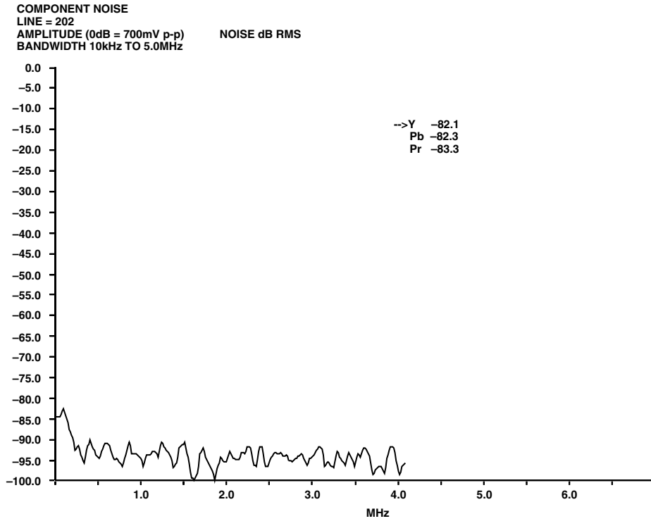
Figure 99. PAL YUV SNR Plot
