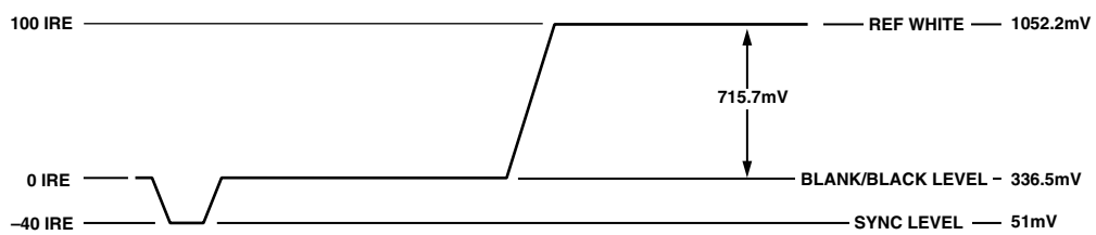
Figure 68. NTSC RGB Video Levels
