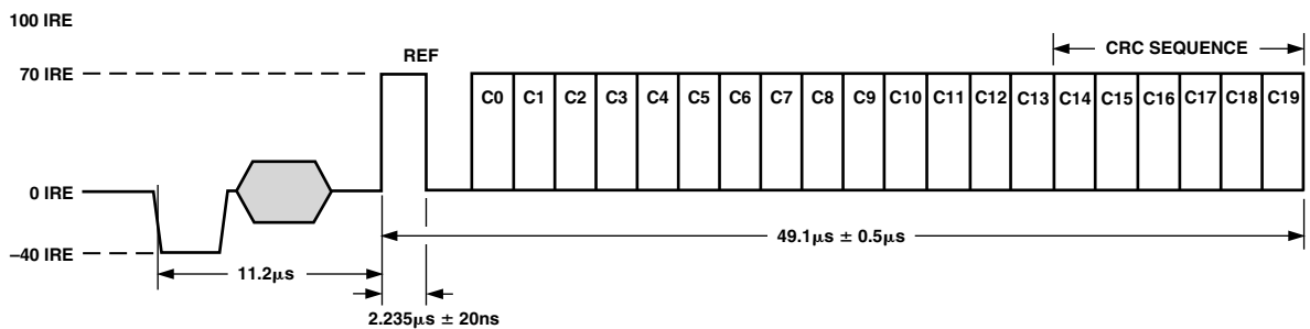
Figure 57. CGMS Waveform Diagram
