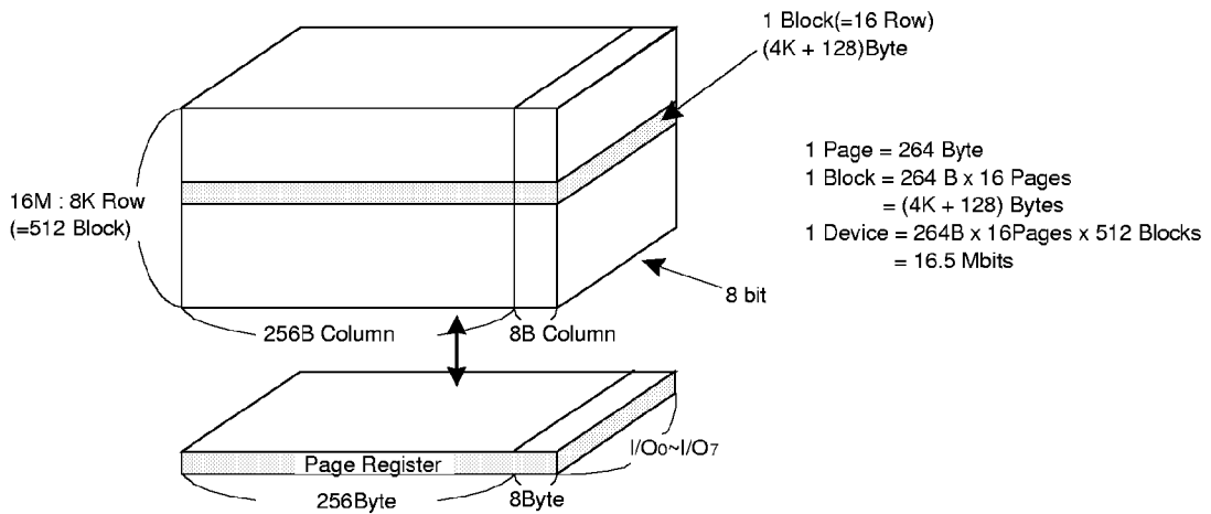
Figure 2. ARRAY ORGANIZATION
