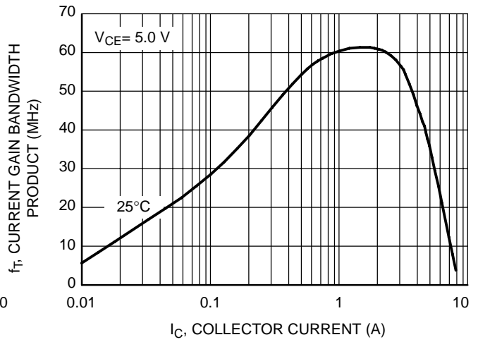
Figure 8. NJL0302A Current Gain Bandwidth Product
