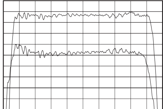
Horizontal: 3.2 MHz/Div Vertical: 1 dB/Div Vertical: 5 deg/Div
