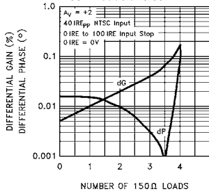
Differential Gain and Phase vs Number of 150 Ohm Loads at 3.58MHz
