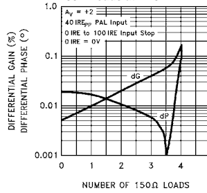
Differential Gain and Phase vs Number of 150 Ohm Loads at 4.43MHz
