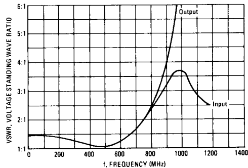
FIGURE 8 – VSWR versus FREQUENCY MWA220
