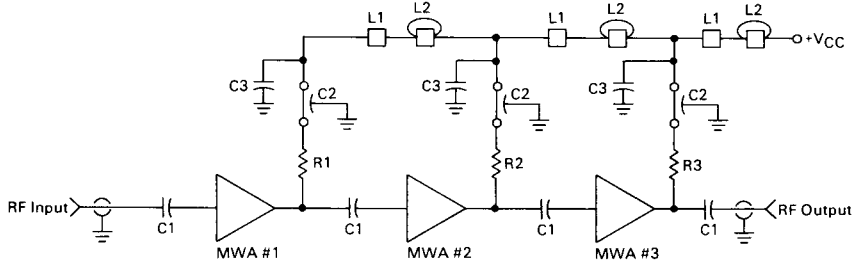
FIGURE 29 — TYPICAL CASCADE
