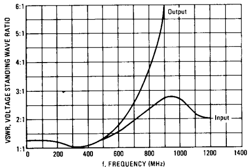
FIGURE 7 – VSWR versus FREQUENCY MWA210
