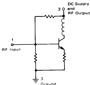
FIGURE 26 – INTERNAL CIRCUIT
