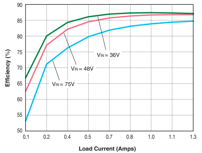
UWR-12/1250-D48A Efficiency vs. Line and Load
