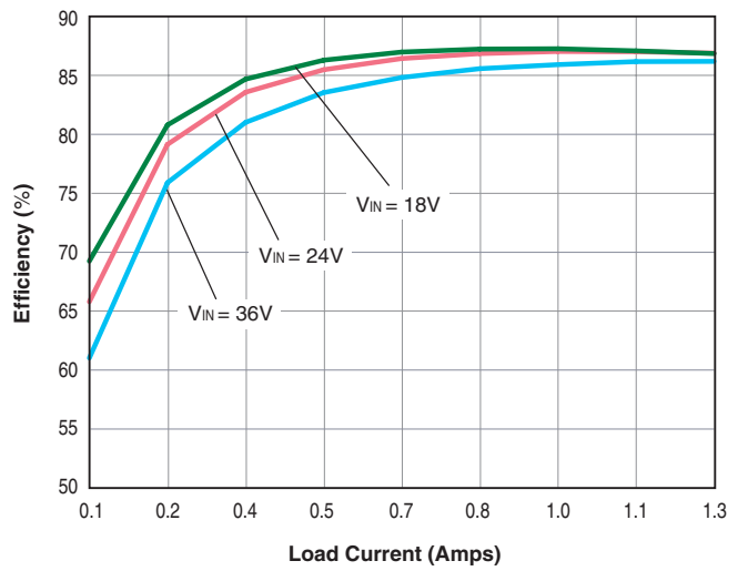
UWR-12/1250-D24A Efficiency vs. Line and Load
