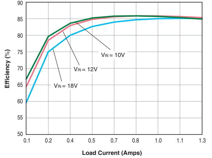
UWR-12/1250-D12A Efficiency vs. Line and Load
