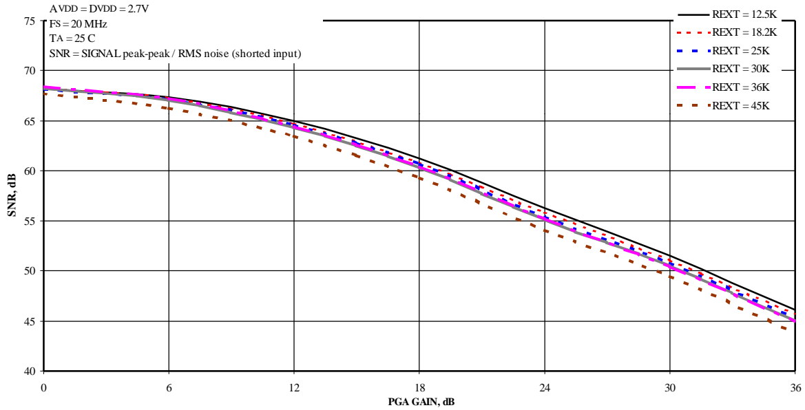
Figure 26. XRD98L61 SNR vs PGA Gain @ 20MHz with Different R EXT
