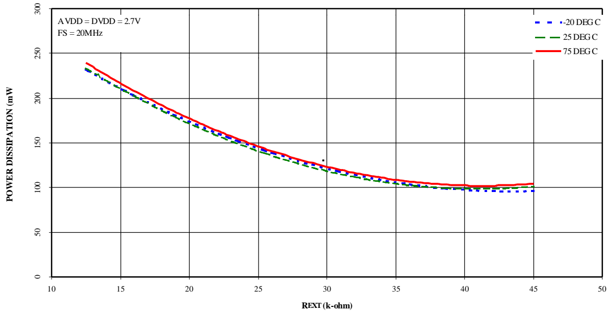
Figure 24. XRD98L61 Power Dissipation vs R EXT @ 20MHz
