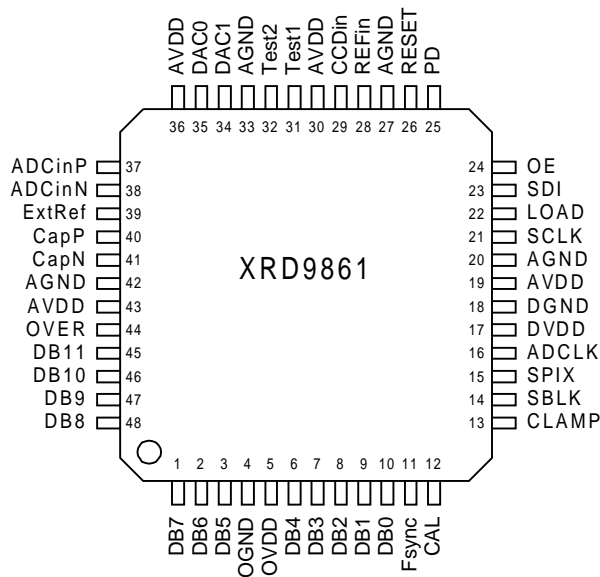
Figure 2. XRD98L61 Pinout
