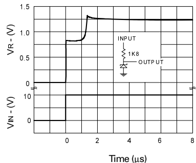
Transient Response ( I_R = 5\text{mA} )
