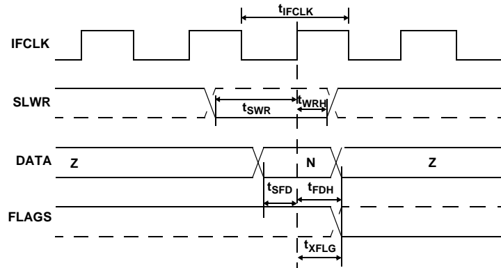
Figure 10-4. Slave FIFO Synchronous Write Timing Diagram [13]
