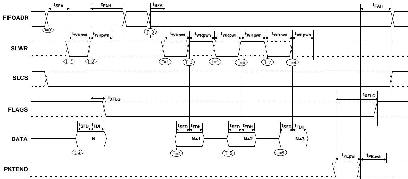
Figure 10-18. Slave FIFO Asynchronous Write Sequence and Timing Diagram [13]
