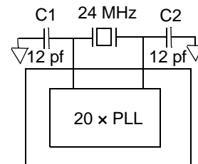
Figure 4-1. Crystal Configuration
