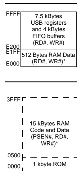
Figure 4-4. Internal Code Memory
