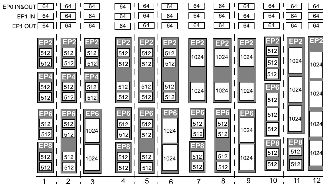
Figure 4-6. Endpoint Configuration
