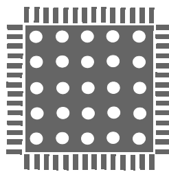
Figure 14-2. Plot of the Solder Mask (White Area)
