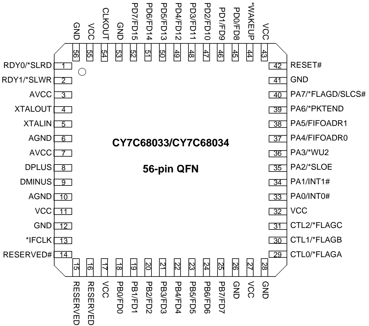
Figure 5-2. CY7C68033/CY7C68034 56-pin QFN Pin Assignment
