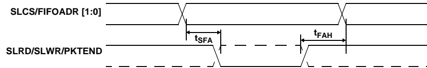
Figure 10-12. Slave FIFO Asynchronous Address Timing Diagram [13]
