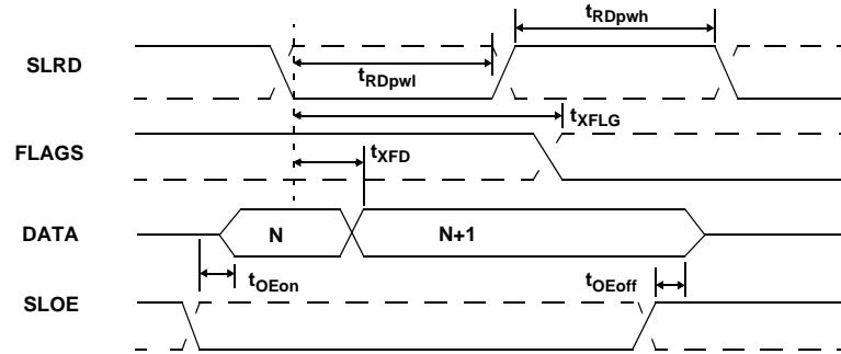
Figure 10-3. Slave FIFO Asynchronous Read Timing Diagram [13]
