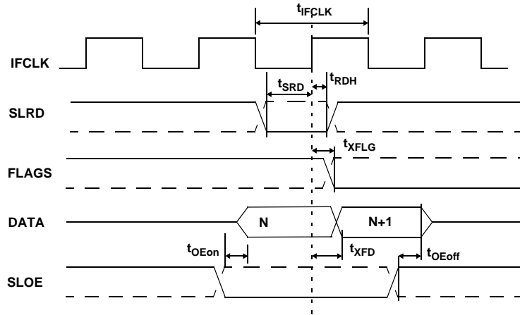
Figure 10-2. Slave FIFO Synchronous Read Timing Diagram [13]
