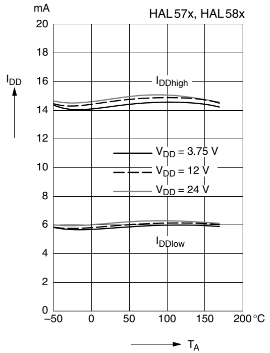
Fig. 3-9: Typical current consumption versus ambient temperature
