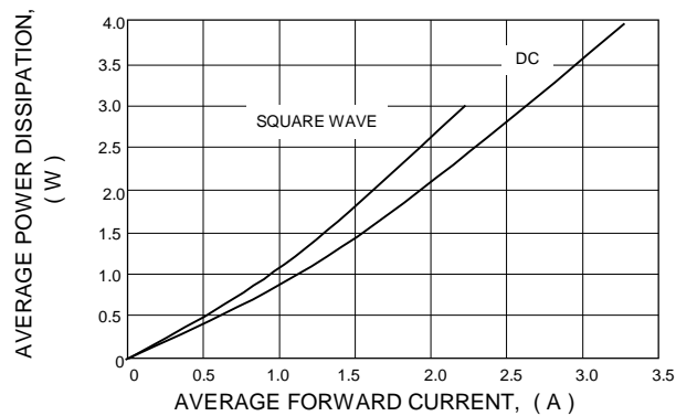
FIG. 5 - POWER DISSIPATION
