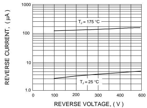
FIG. 4 - MAXIMUM REVERSE CURRENT
