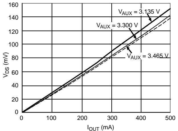
Figure 26. PFET V_{DS} vs. I_{OUT}
