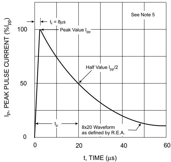
Fig. 4 Pulse Waveform
