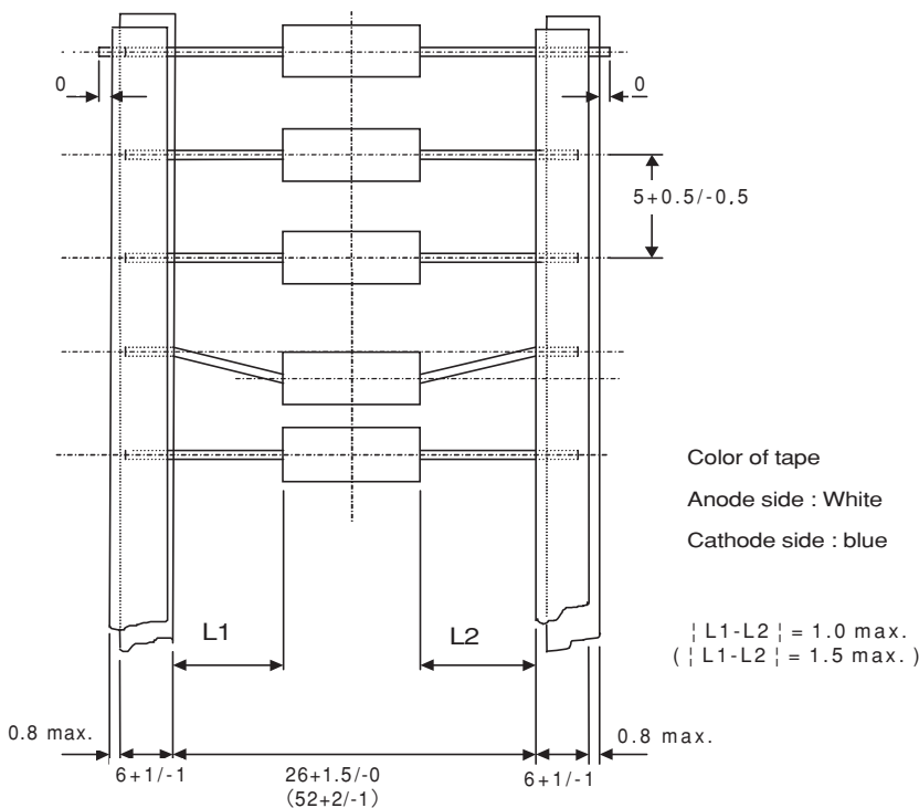
Axial Taping
