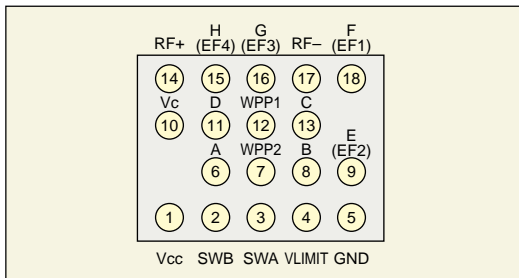
■ Figure 4 CXA2702GA Pin Configuration (Items in parentheses apply to the CXA2716GA.)
