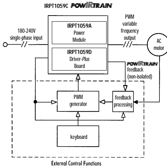
Figure 2. The IRPT1059C POWIRTRAIN within a motor control system
