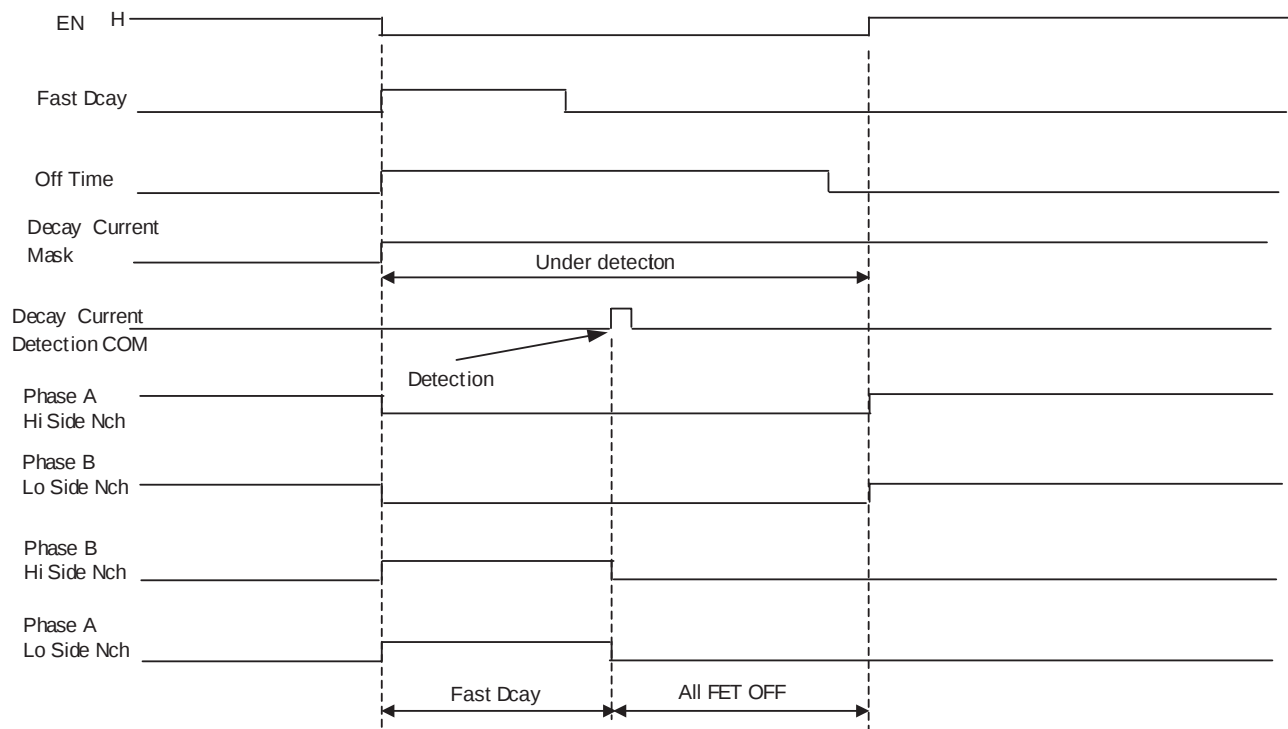
External PWM Sync.Rect.Enable Control1 "H" Fast Decay
