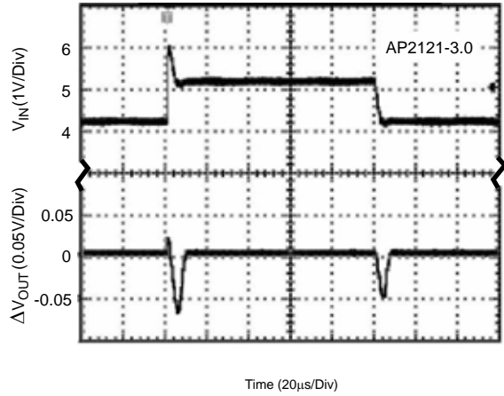
Figure 17. Line Transient (Conditions: I_{OUT}=30mA , C_{IN}=1\mu F , C_{OUT}=1\mu F )
