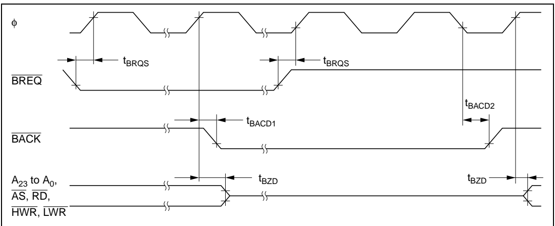
Figure 21.18 Bus-Release Mode Timing
