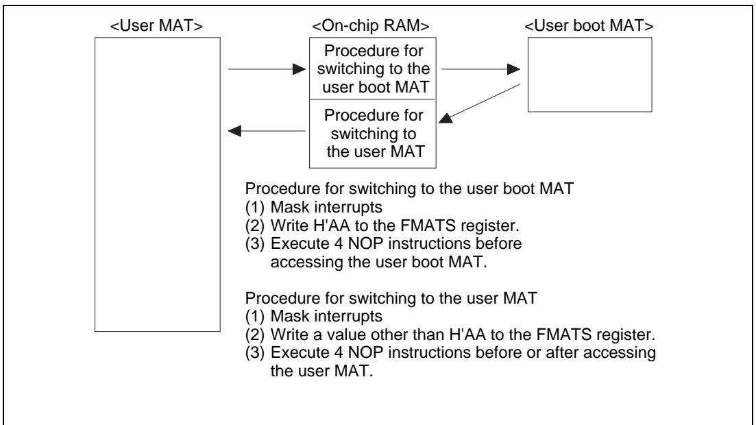
Figure 18.20 Switching between the User MAT and User Boot MAT
