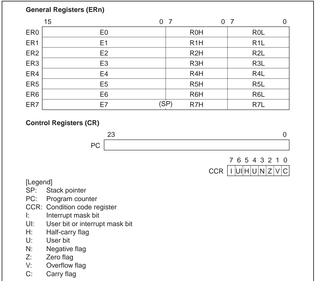
Figure 2.3 CPU Registers
