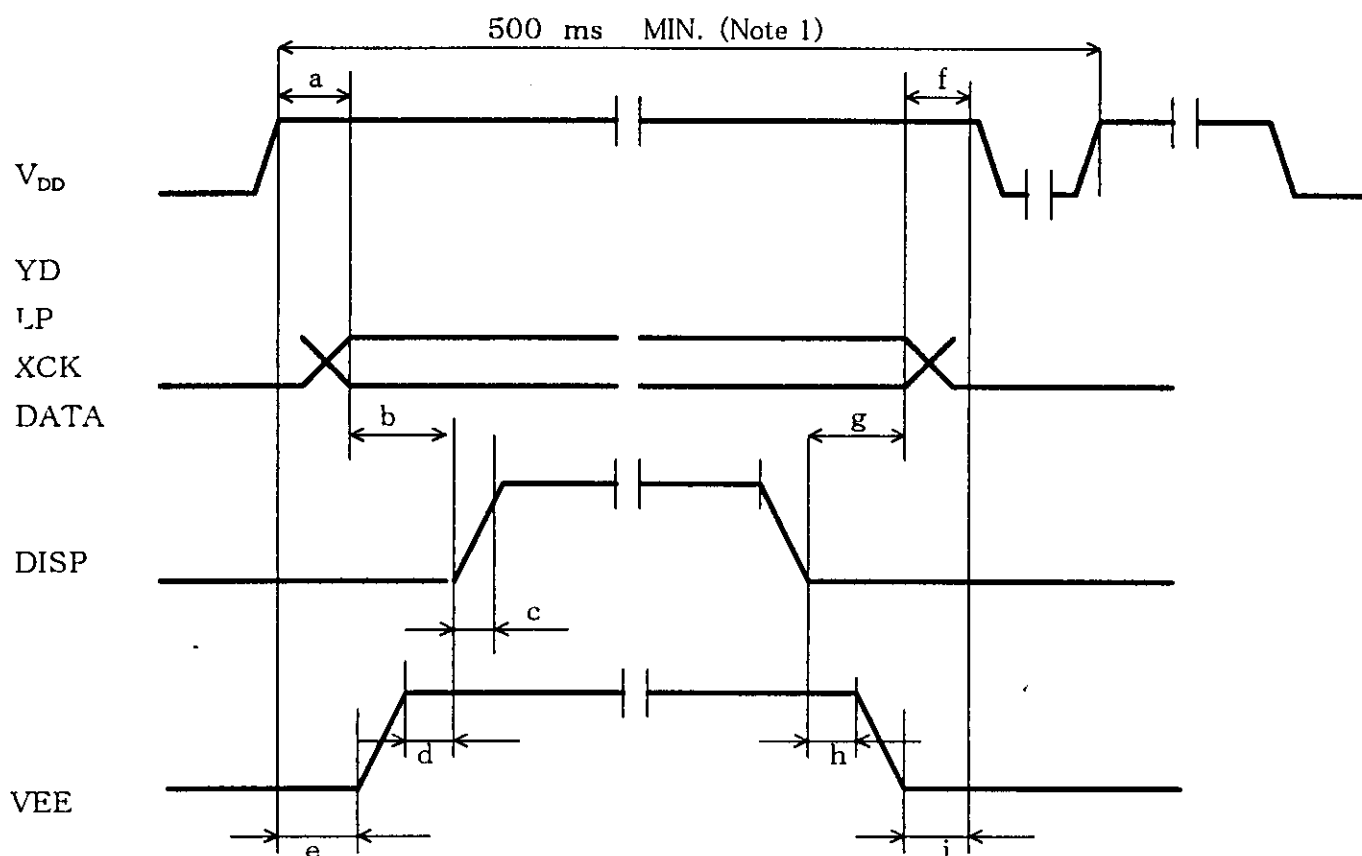
Fig. 12 Sequence condition
