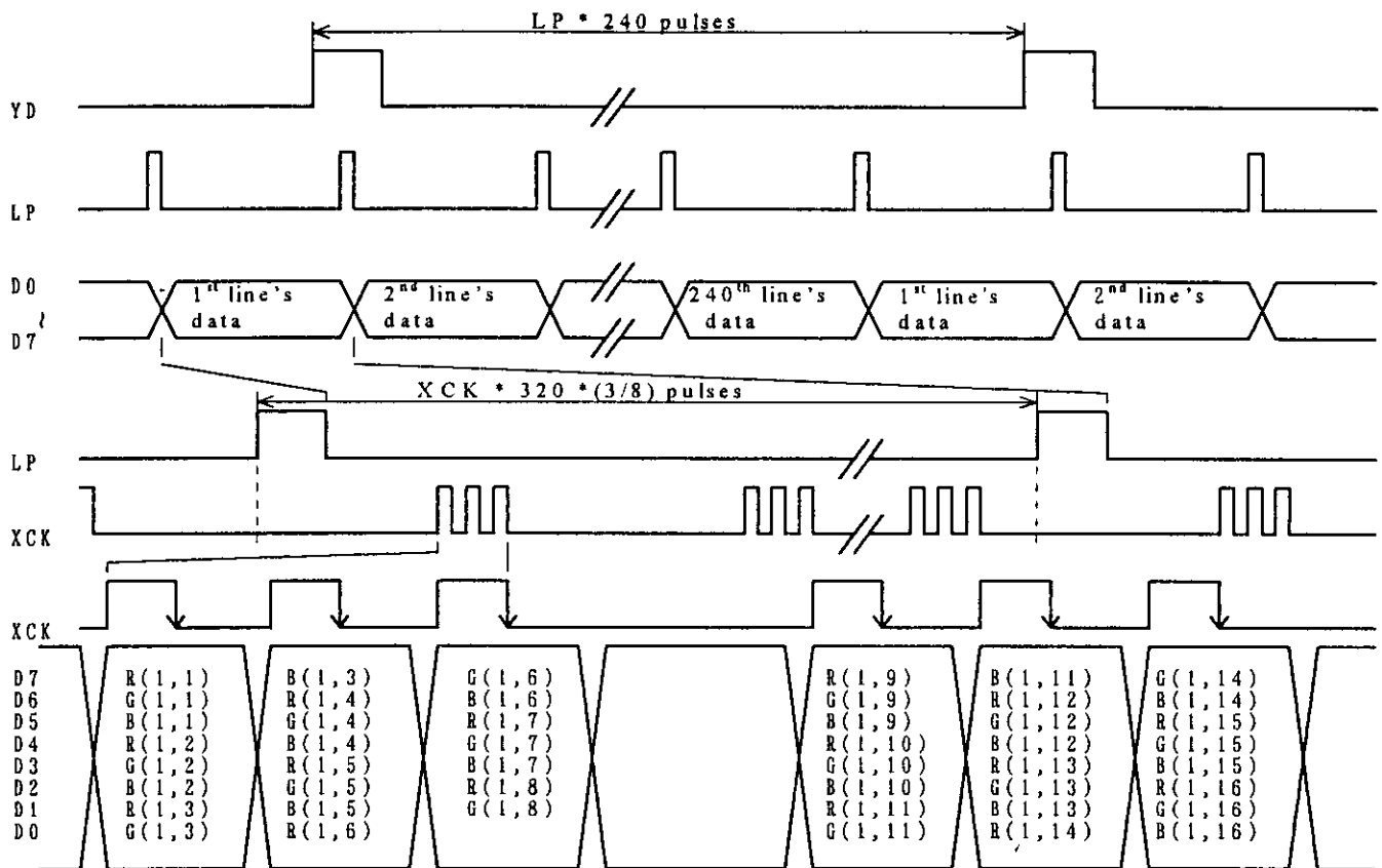
Fig.2 Interface timing
