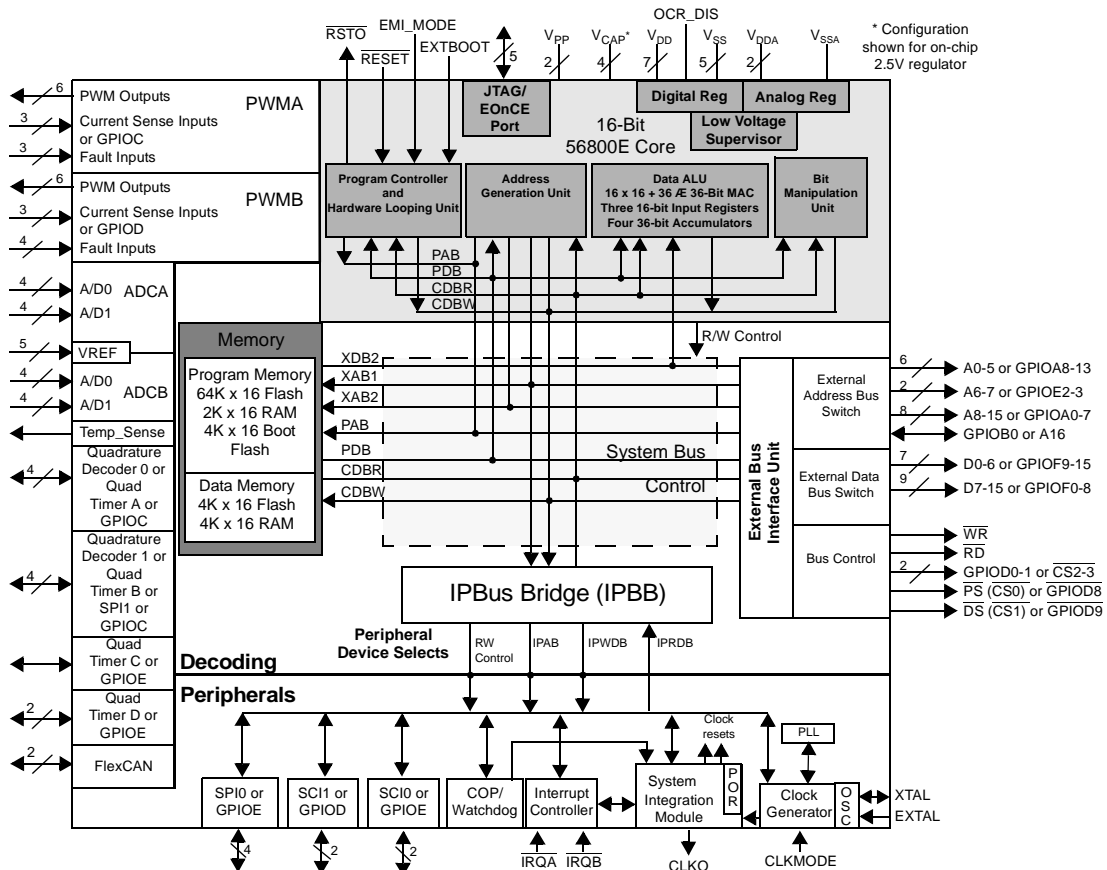
56F8346 Block Diagram
