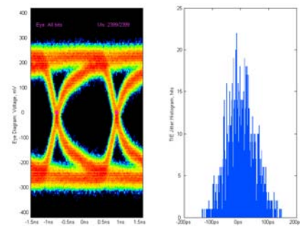
Figure 57. Data Eye for LVDS Outputs in ANSI Mode with 100 Ohm Termination on and Trace Lengths of Greater than 24 Inches on Standard FR-4
