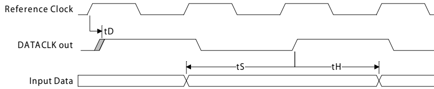
Figure 34. Timing Specifications for AD9776, PLL Enabled, Reference Clock = 2x Input Sample Rate
