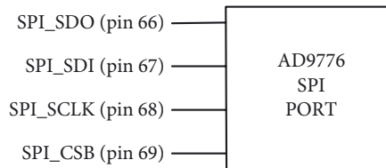
Figure 24. AD9776 SPI Port
