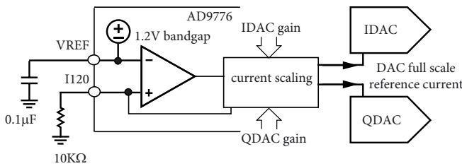
Figure 29. Reference Circuitry
