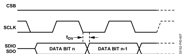
Figure 28. Timing Diagram for SPI Register Read
