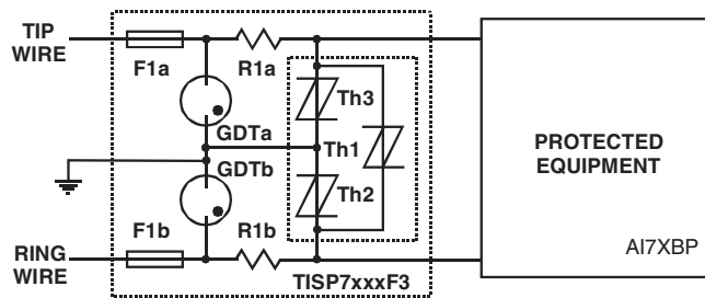
Figure 21. Protection Module
