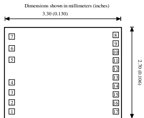
Figure 2 Pad location on XE2004I-000 (not to scale)
