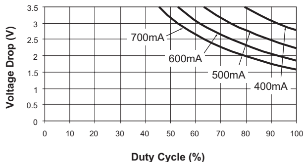
Device Duty Cycle vs. V_{DROP} ( V_{OUT} = 1.5V @ 25^\circ C )
