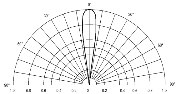
Relative Brightness (LOP@MAX.=1)
