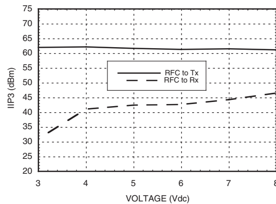
Input IP3 vs. Voltage with 2600 MHz Tuning
