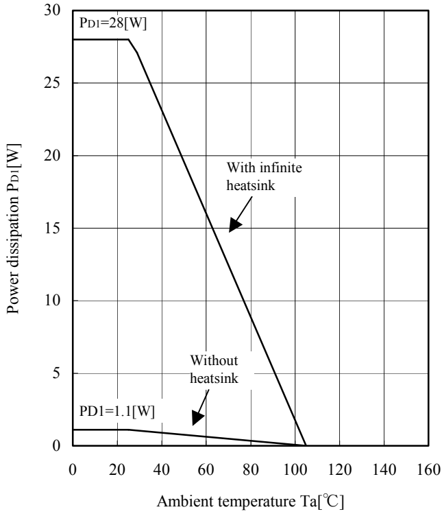
IRIS-W6754 MOSFET Ta-PD1 Curve
