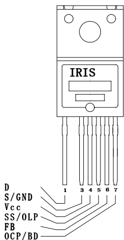
Pin Assignments
