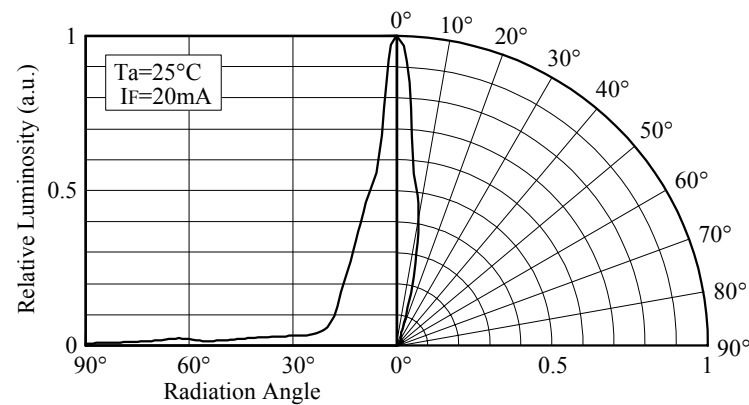
■ Directivity (NSPB300A)
