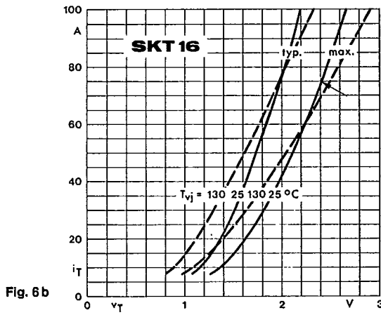
Fig. 6 b On-state characteristics
