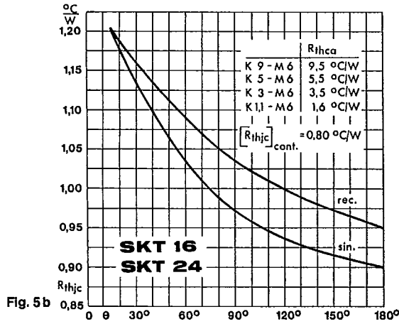
Fig. 5 b Thermal resistance vs. conduction angle
