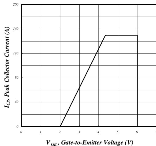
Fig 6. Minimum Gate Drive Area
