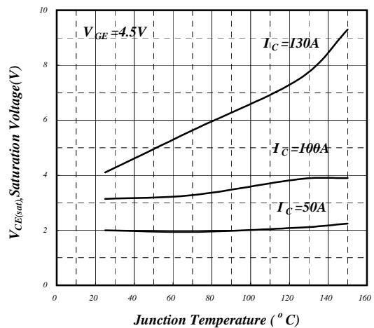
Fig 4. Collector-Emitter Saturation Voltage v.s. Junction Temperature
