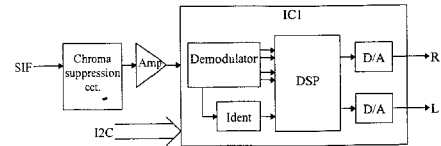
Block diagram of the NICAM/A2
