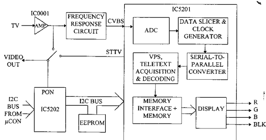
Block diagram of Teletext decoder
