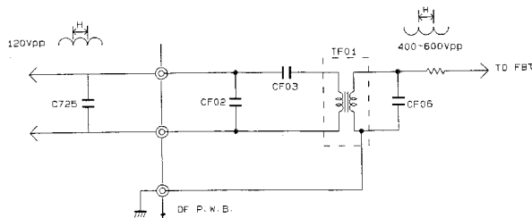
DYNAMIC FOCUS PWB CIRCUIT
