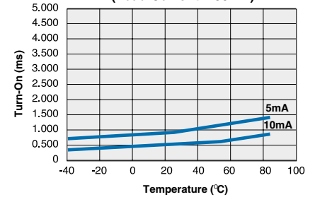
CPC1135N Typical Turn-On vs. Temperature (Load Current = 50mA)
