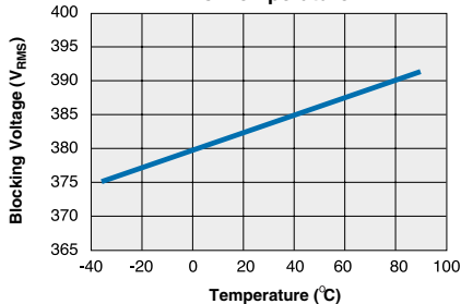
CPC1135N Typical Blocking Voltage vs. Temperature
