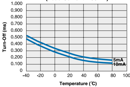
CPC1135N Typical Turn-Off vs. Temperature (Load Current = 50mA)
