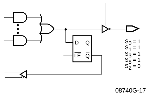
Output Combinatorial/Active Low, Latched Feedback
