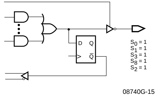
Output Combinatorial/Active Low, Register Feedback
