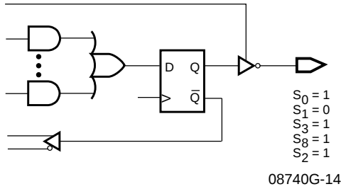
Output Registered/Active Low, Register Feedback
