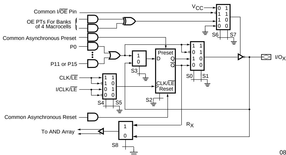
Figure 2a. PALCE29M16 Macrocell (Single Feedback)
