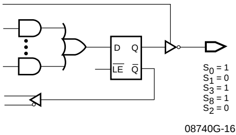
Output Latched/Active Low, Latched Feedback
