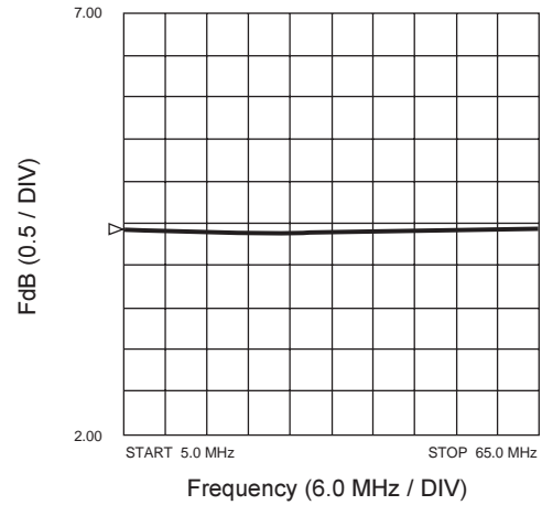
NOISE FIGURE
