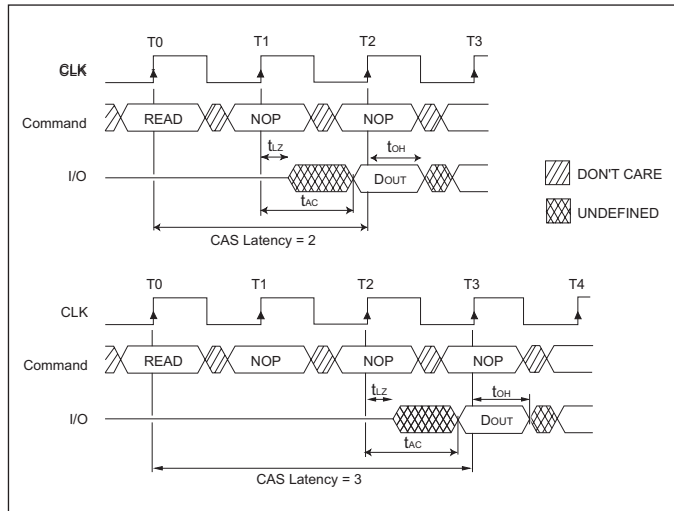
FIGURE 4 – CAS LATENCY
