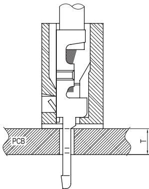
TERMINAL ASSEMBLY DRAWING
