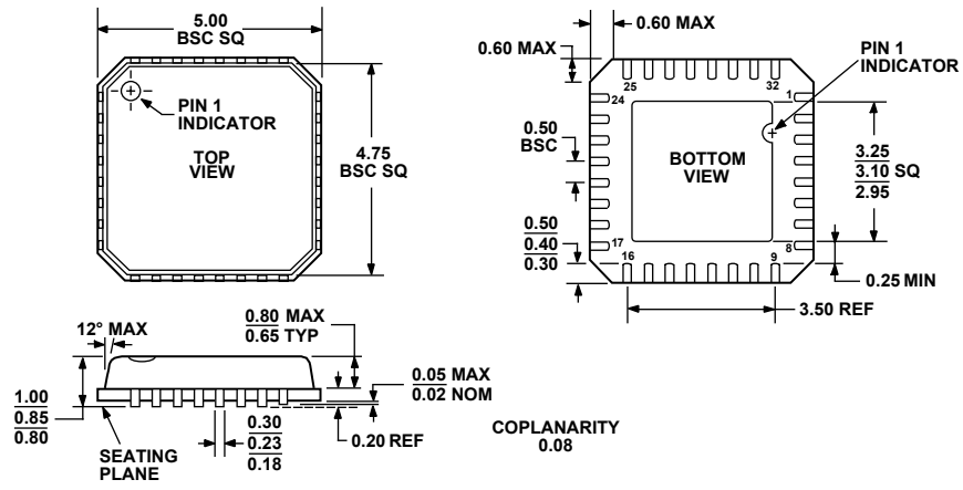
Figure 21. 32-Lead Frame Chip Scale Package [LFCSF] (CP-32) Dimensions shown in millimeters
