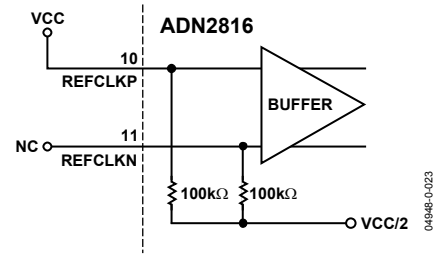
Figure 17. No REFCLK Configuration
