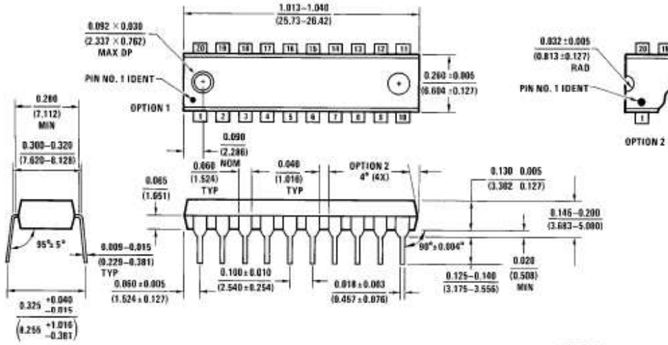
Molded Dual-In-Line Package (N)
