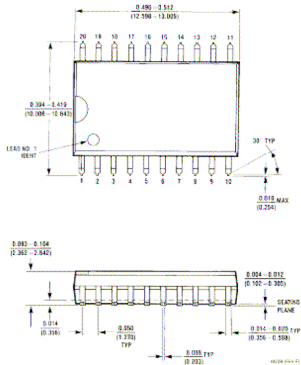
Molded Small Outline Package (WM)
