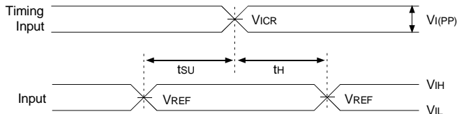
Voltage Waveforms - Setup and Hold Times
