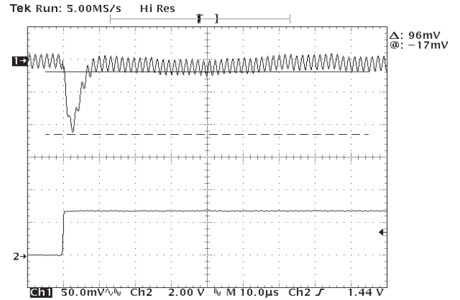
Figure 24: Transient Response 70% - 100% (Channel 2: Current Step at 2.5 A/div, Channel 1: Output Voltage Deviation)
