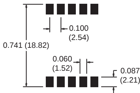
Suggested PCB Pad Layout
