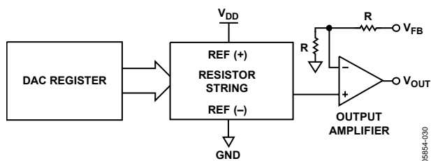
Figure 22. DAC Architecture
