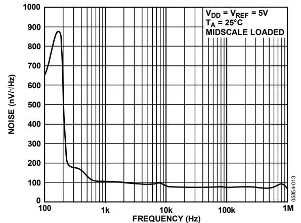
Figure 21. Noise Spectral Density
