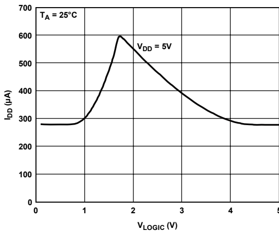
Figure 12. Supply Current vs. Logic Input Voltage
