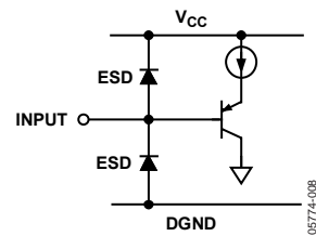
Figure 9. Logic Input
