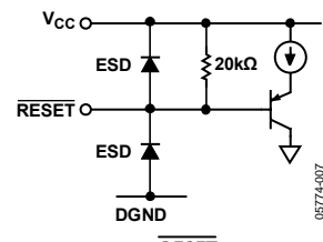
Figure 8. RESET Input
